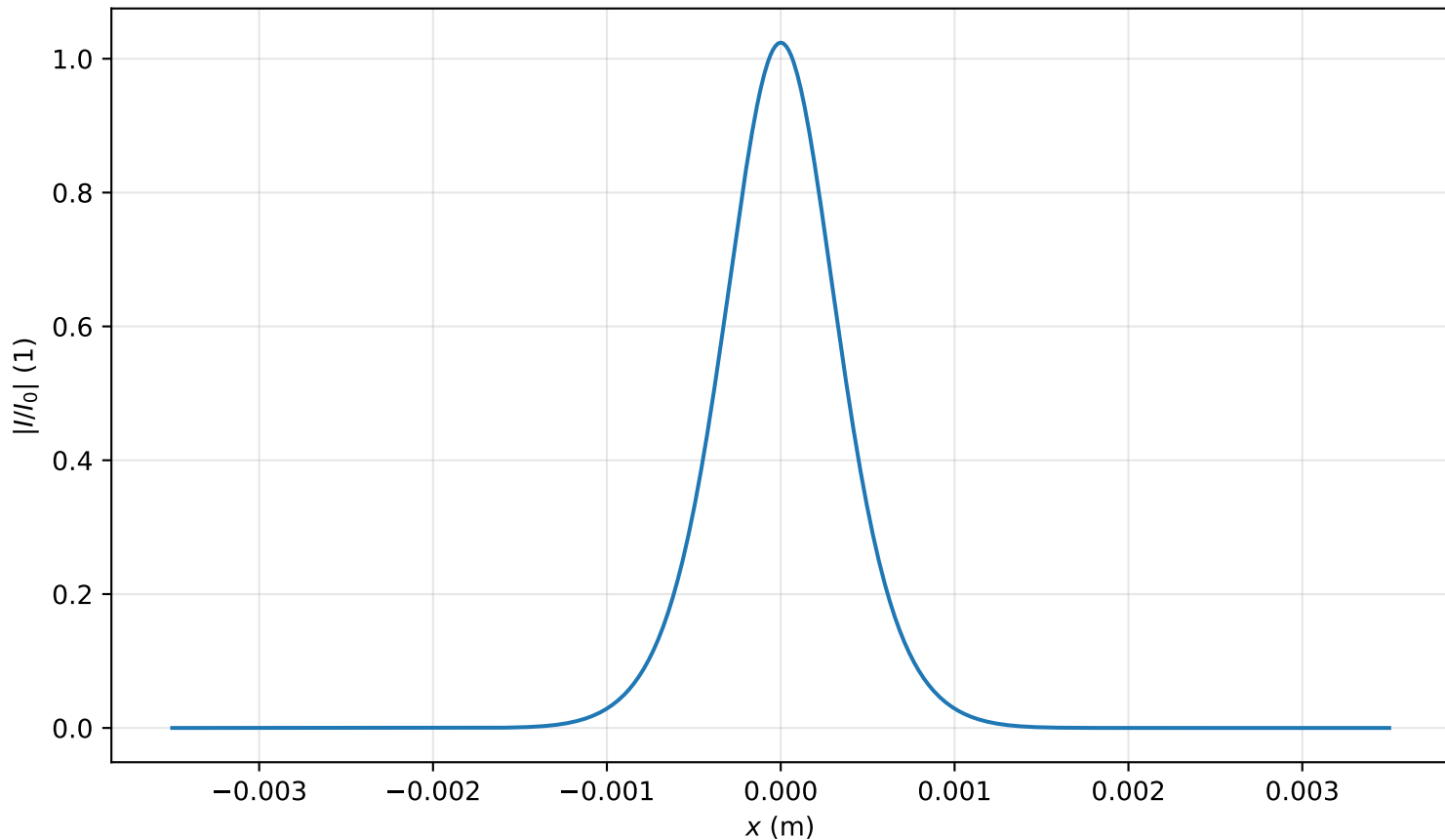
Intensity profile I(x, y = 0, z = 1.194m)/I_0 , \text{Pin}=0.5\text{Pcr} , artificial time
